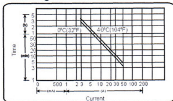
Discharge Current vs Time
